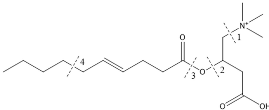
Fragmentation of 4-decenoylcarnitine.
