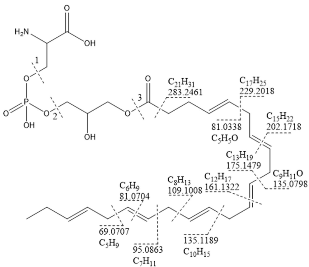
Fragmentation of LysoPS(22:6)
